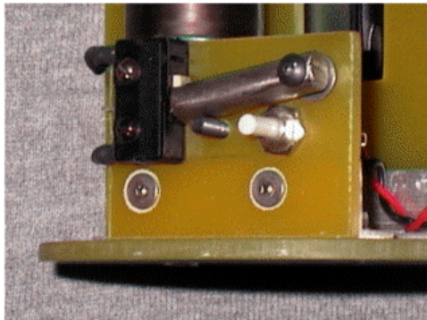
Newer version of the rocket camera, built entirely from 1/8" G10 fiberglass. Same basic design with the gearmotor, cam, and lever, but with a neat little "G" switch made from a microswitch and piece of round stock.
