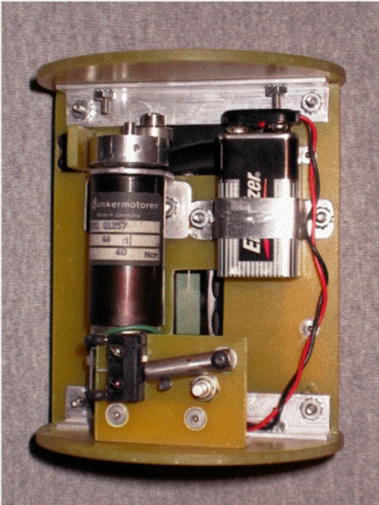
Newer version of the rocket camera, built entirely from 1/8" G10 fiberglass. Same basic design with the gearmotor, cam, and lever, but with a neat little "G" switch made from a microswitch and piece of round stock.
